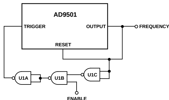
Figure 8. The AD9501 Configured as a Programmable Oscillator
